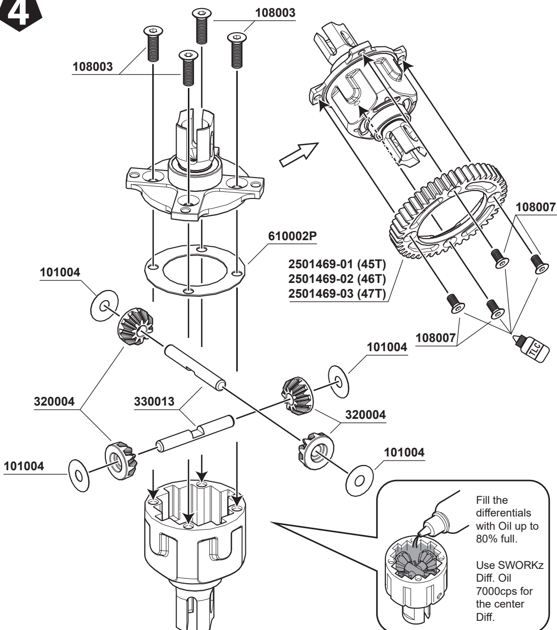
108003 M3x10mm FH/ST HEX Screw x4
