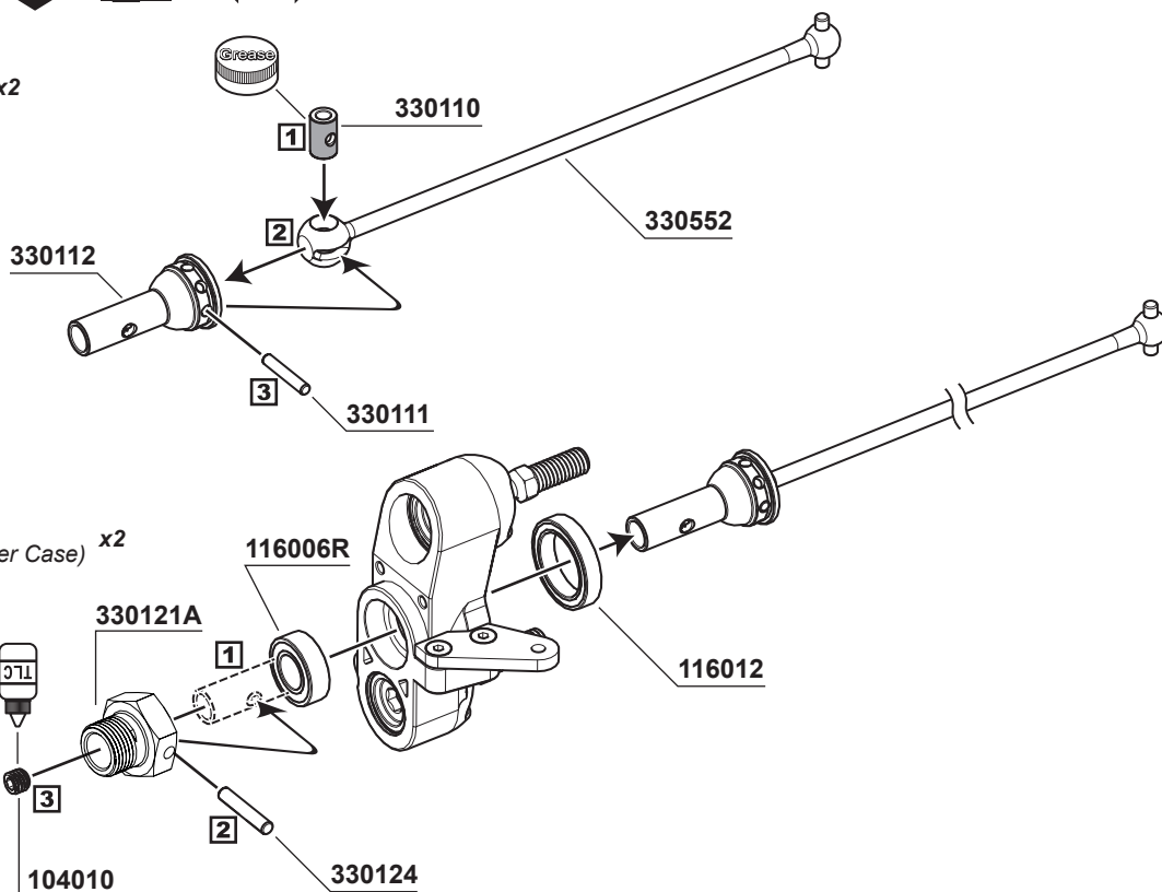
116012 Ball Bearing 15x21x4mm
