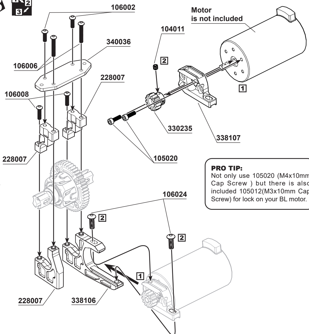
106008 M3x12mm Hex Socket OH/TP Screw x2
