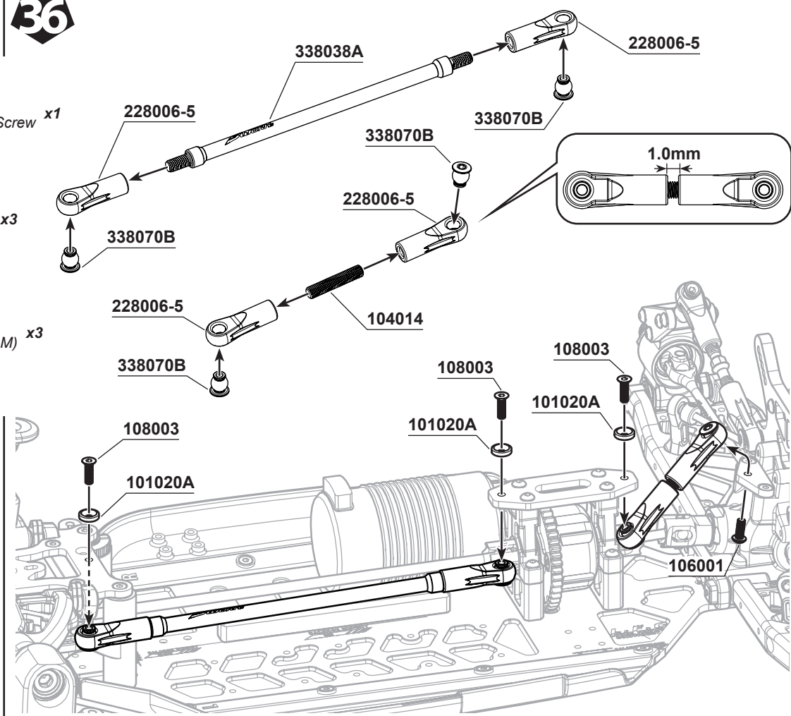
104014 M5X25mm set screw x1
